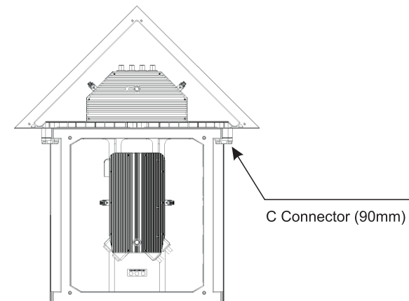
Figure 3.1.3 Design sketch 2 of triangles cabinet connection
