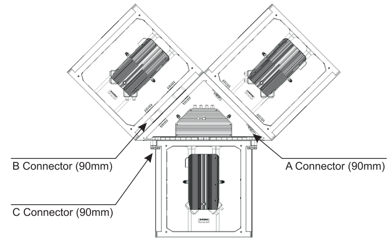
Figure 3.1.2 Design sketch 1 of triangles cabinet connection
