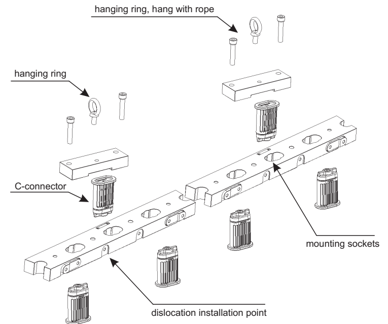
Figure 3.1.1.1 Aluminum hanging beam installation diagram
