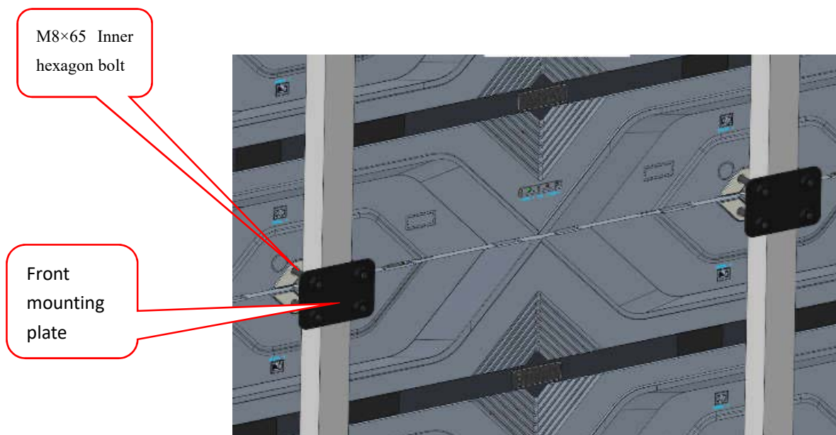
Fig 2-6 Back view of front maintenance Installation Details
