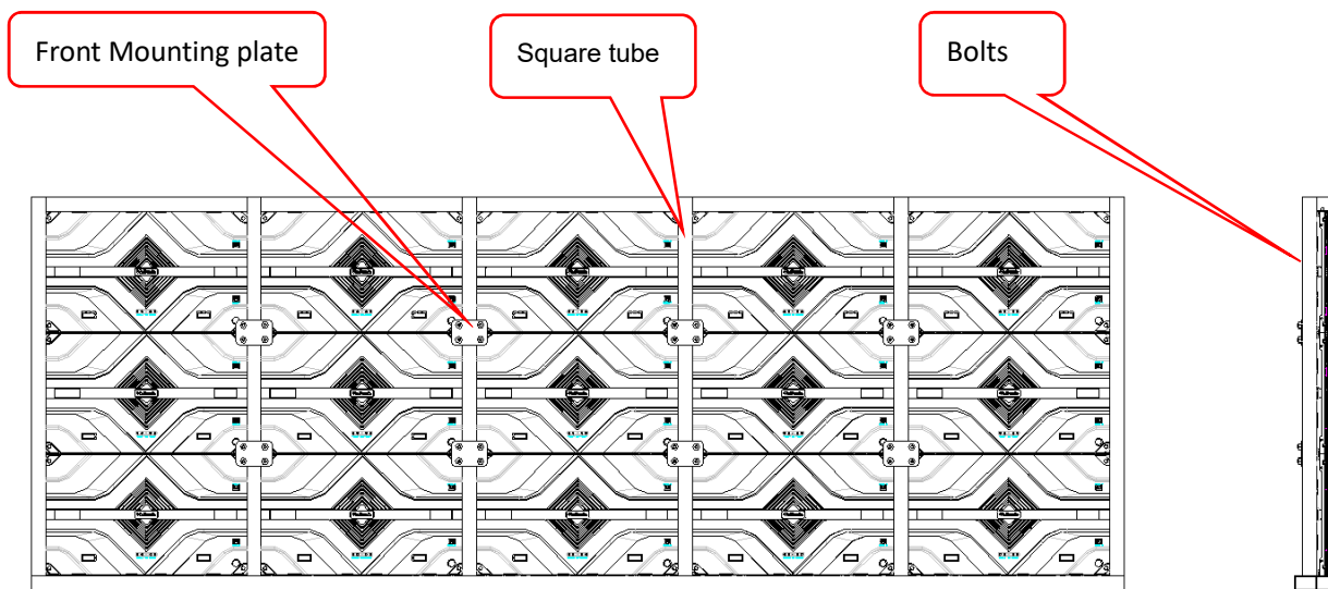
Fig 2-7 Back view of front maintenance Installation
