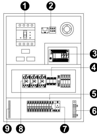
Fig 2-19 Internal Structure of Distribution Box
