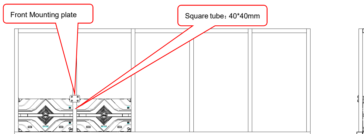
Fig 2-3 Cabinet Fastening
