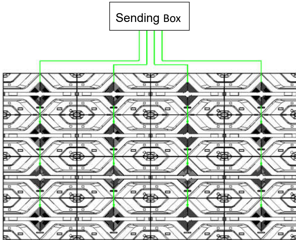
Fig 2-17 Signal Cable Connection Diagram of EasyNATURAL 1.2
