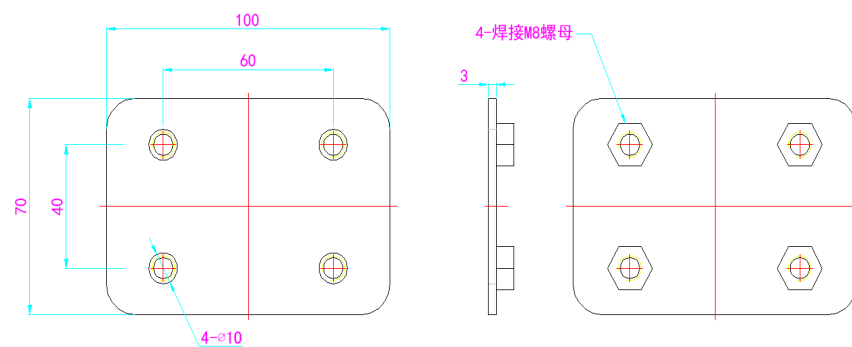
Fig 2-4 Front Connecting Plate
