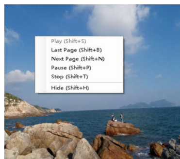
Fig 4-25 Short-cut Menu
