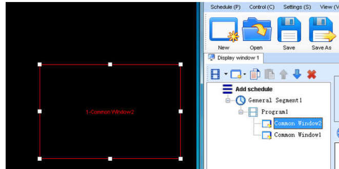
Fig 4-12 Added Window
