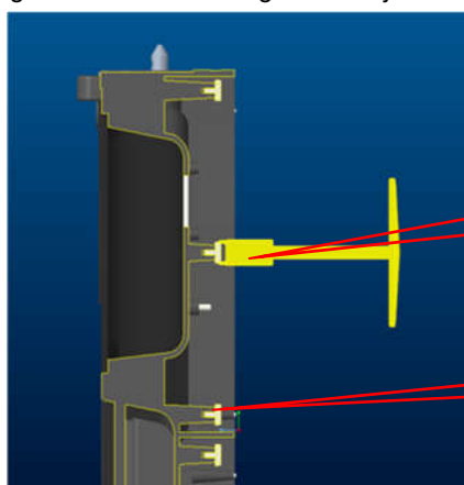
Fig 2-16 Schematic diagram of module flatness adjustment
