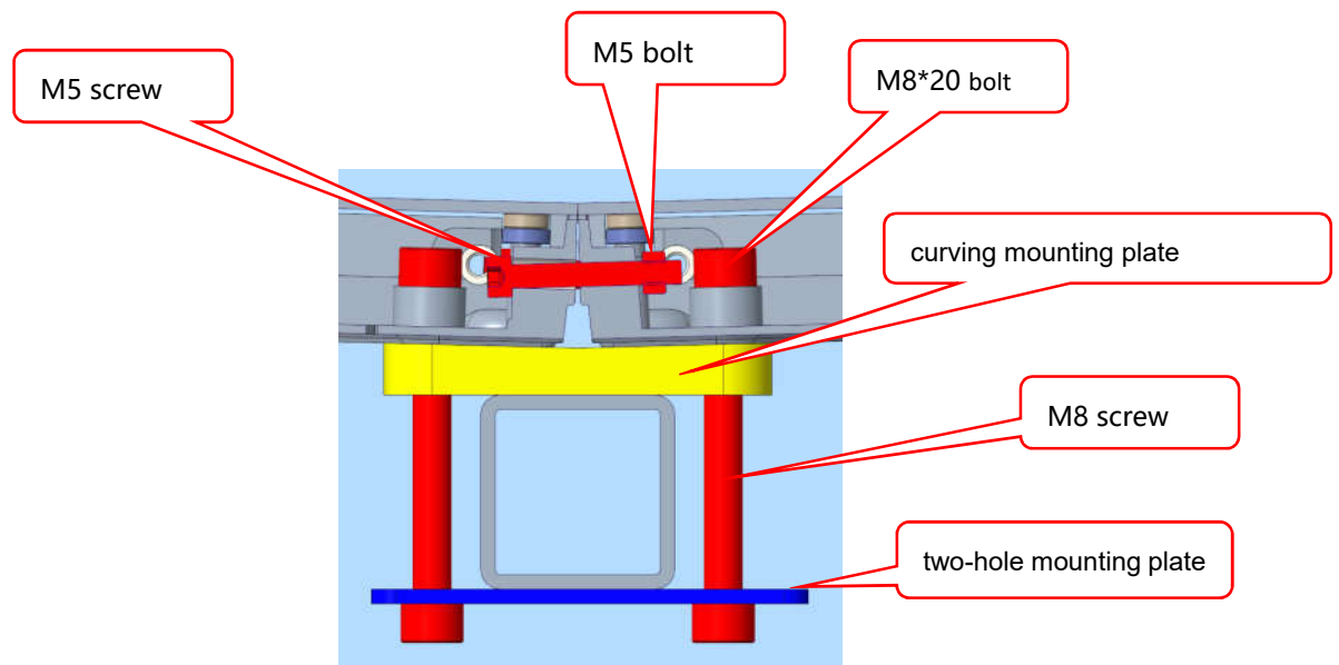
Fig 2-10 concave curving installation
