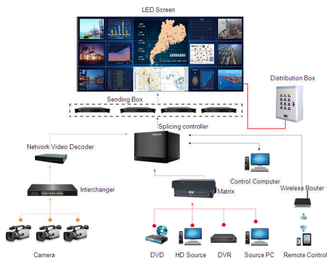
Fig 1-2 System Topology
