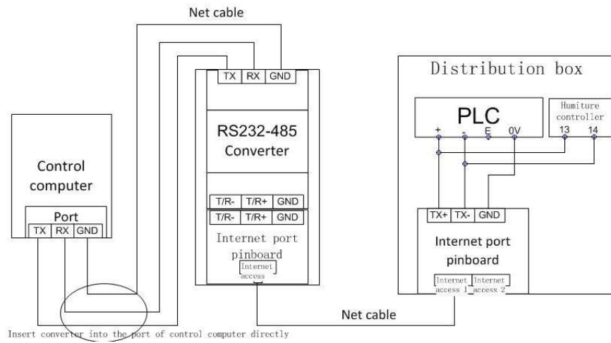
Fig 2-20 Distribution Box PLC Connection Diagram
